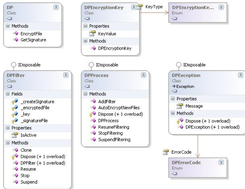
Fig. 4.1: DP4NET classes
